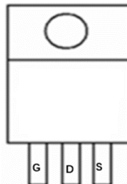
Pin Assignment
